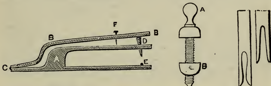
FIG. 128.—Gauging Callipers.
